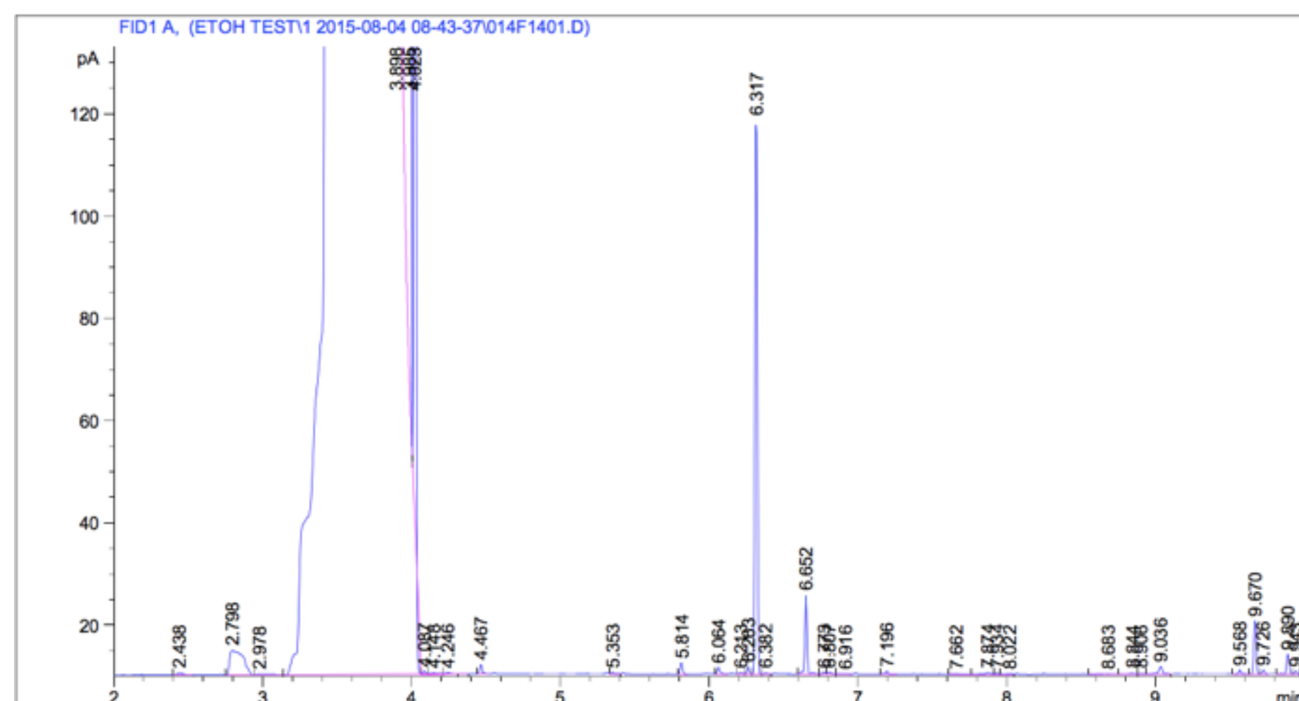
Terpenoid Distribution
