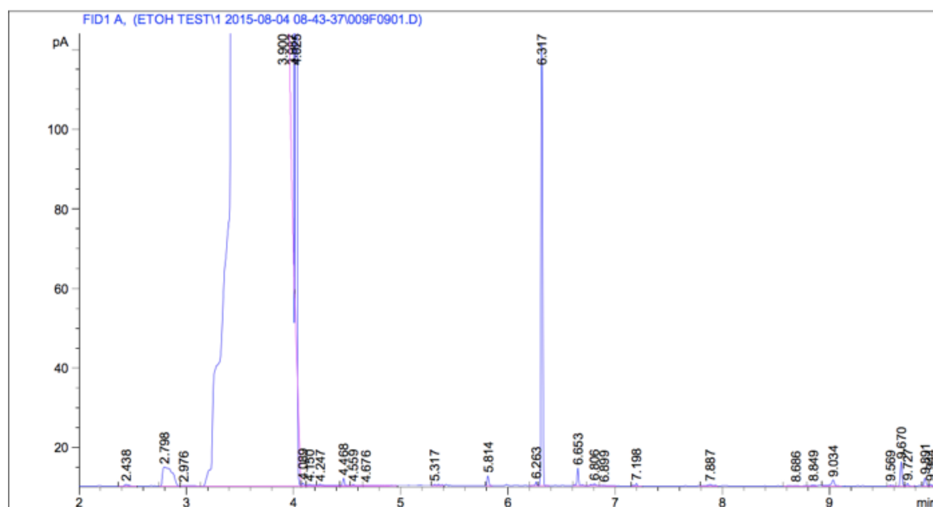
Terpenoid Distribution
