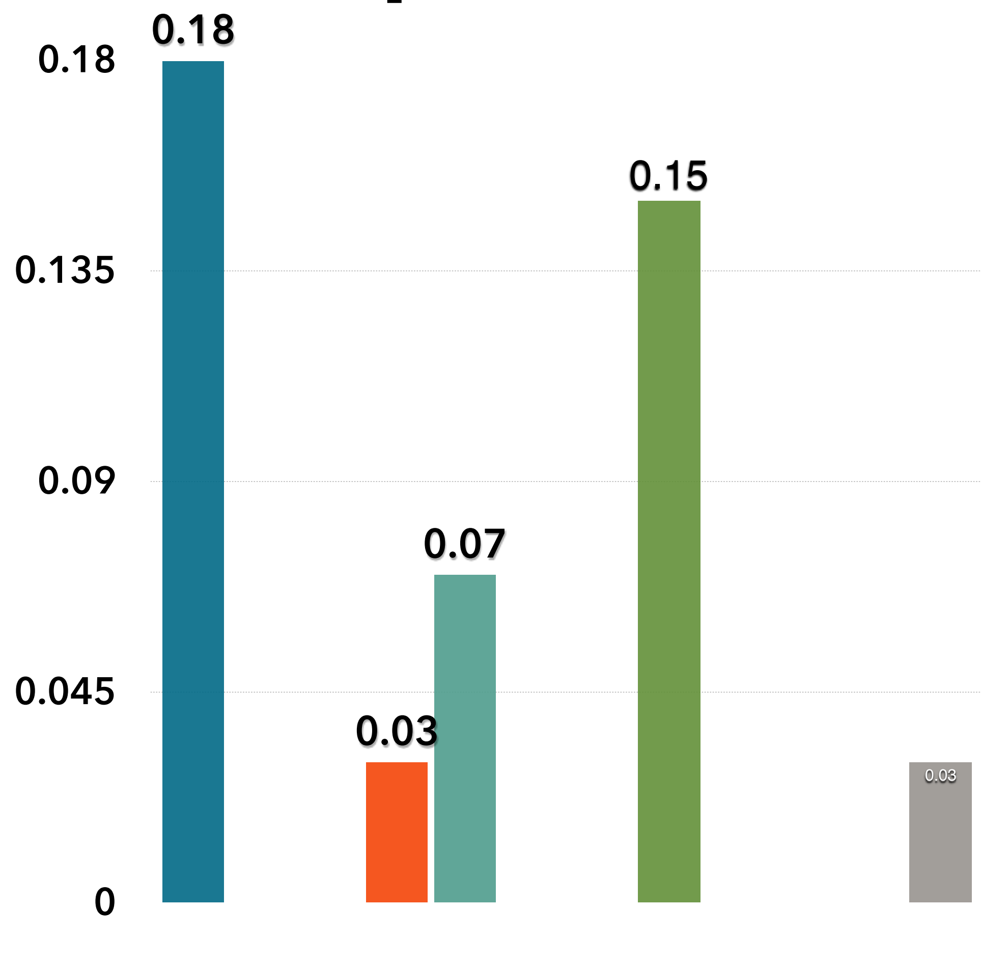
Terpenoid Distribution
