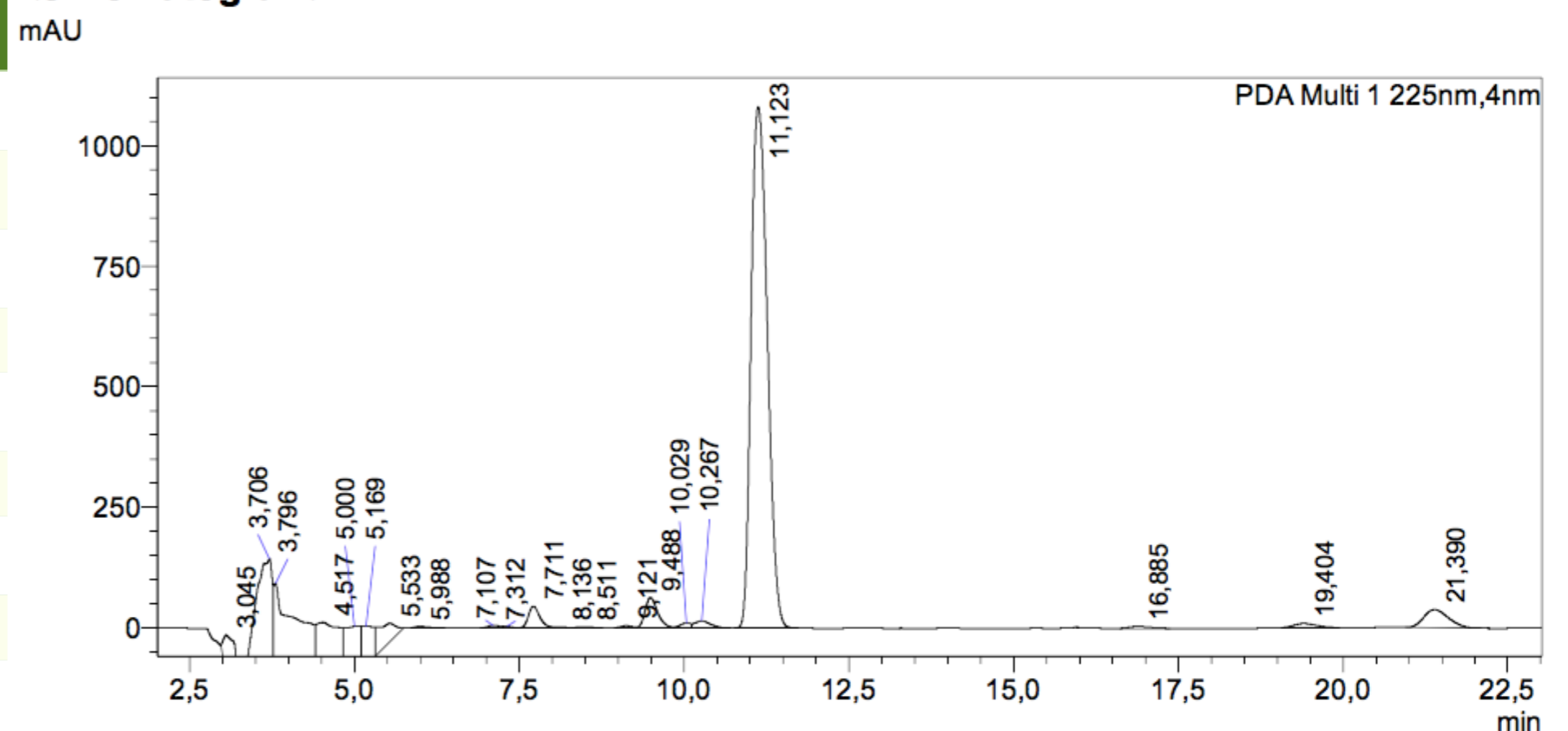
<Chromatogram>
