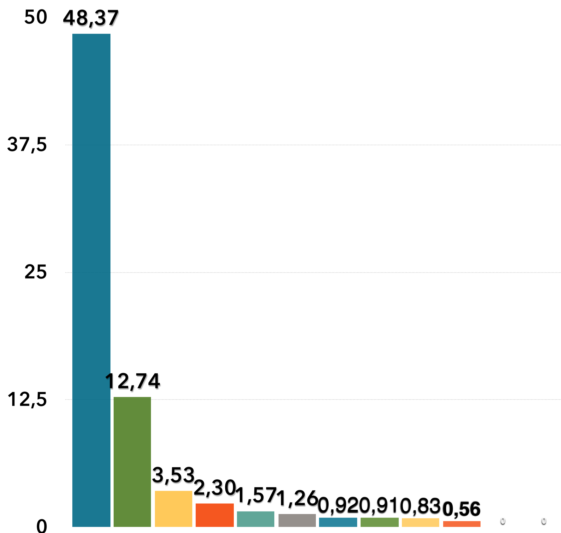
Terpenoid Distribution
