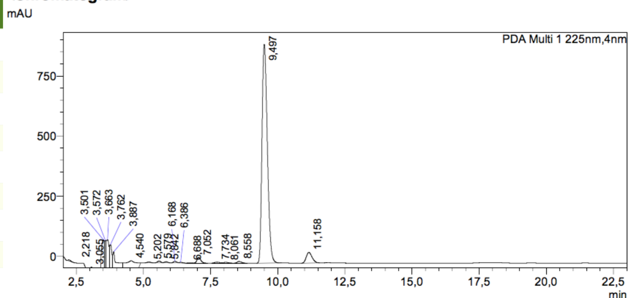
<Chromatogram>
