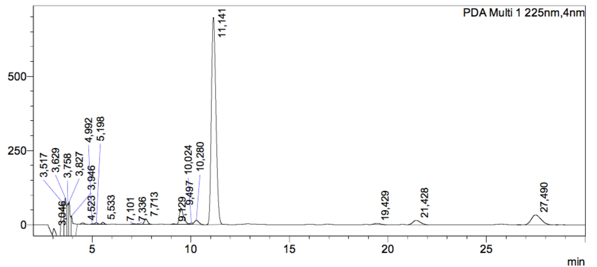
<Chromatogram> mAU
