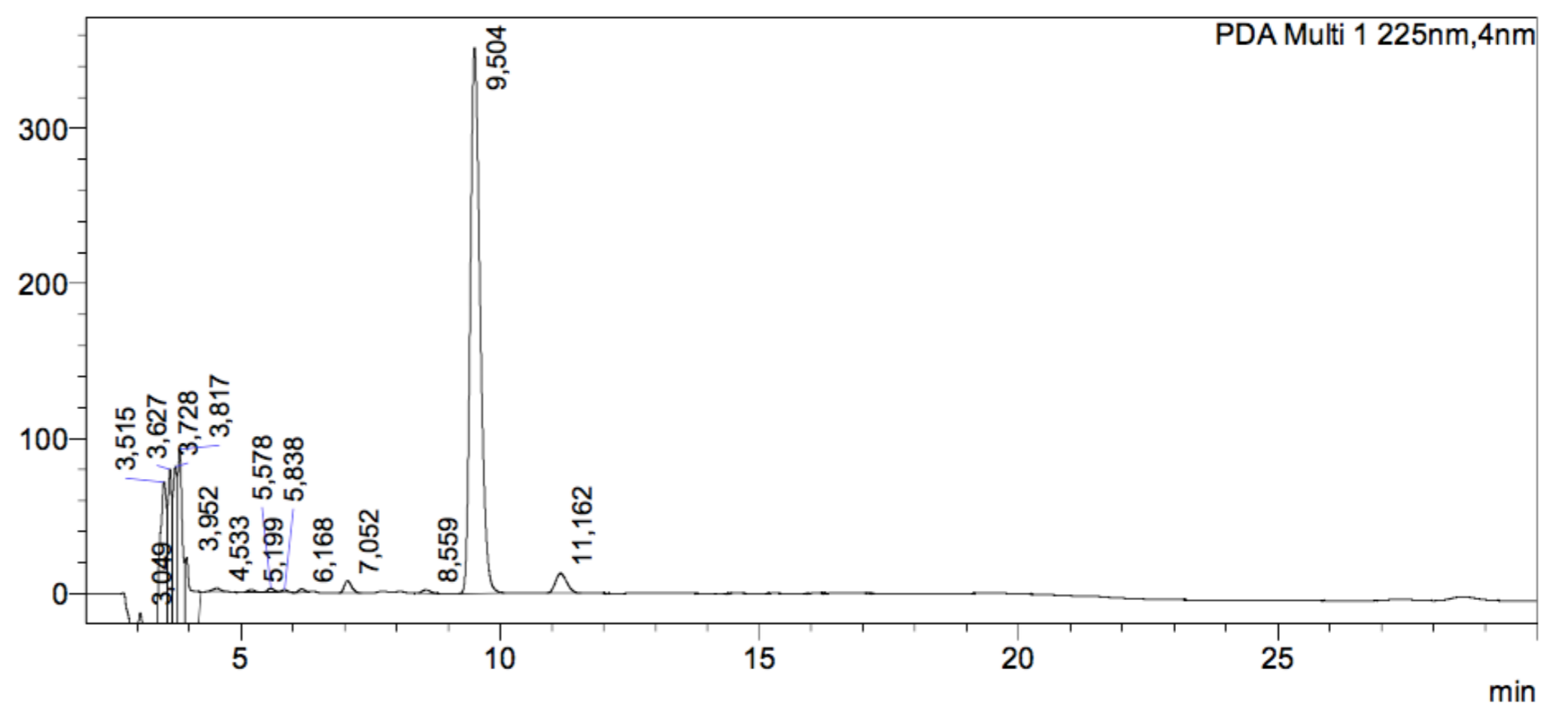
<Chromatogram> mAU
