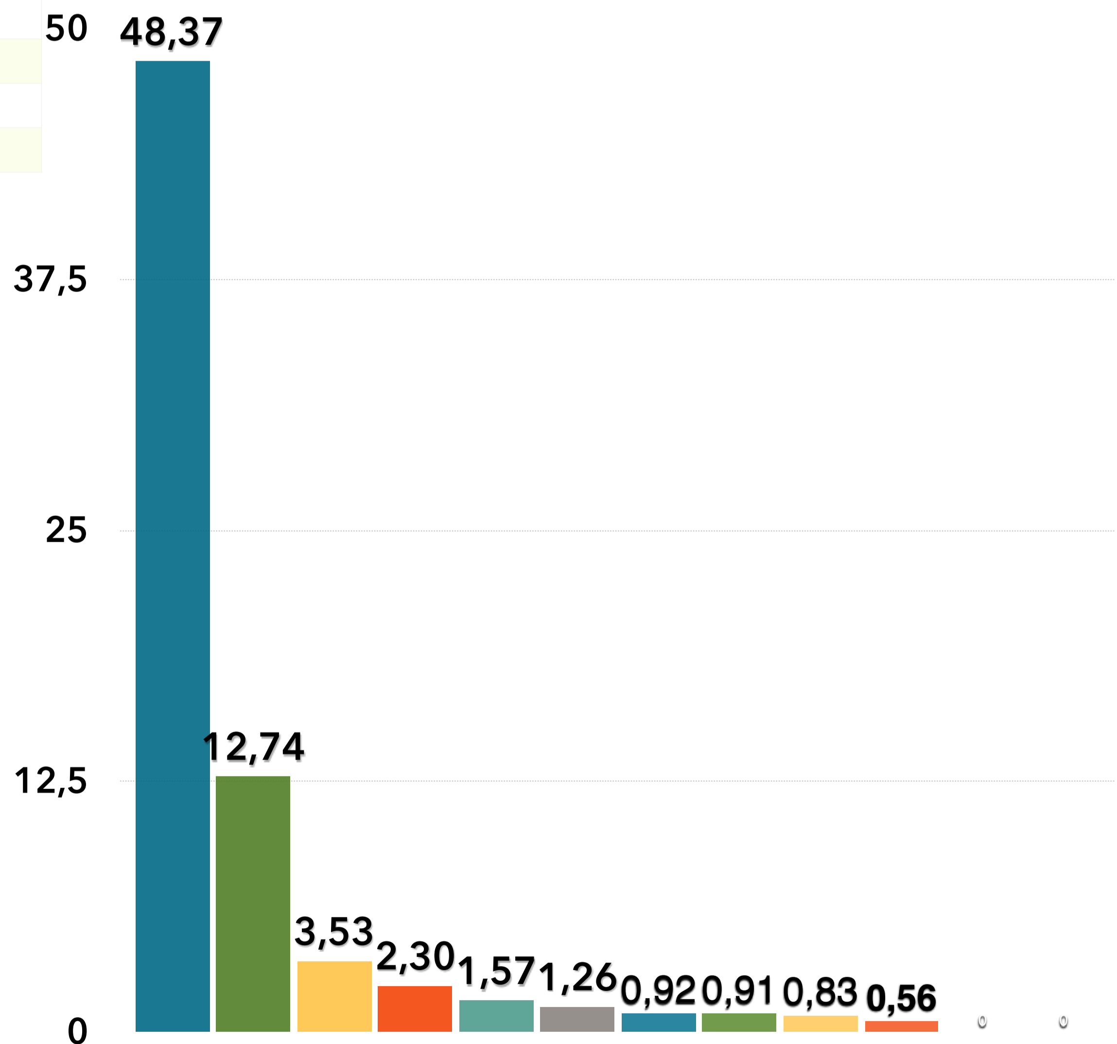
Terpenoid Distribution
