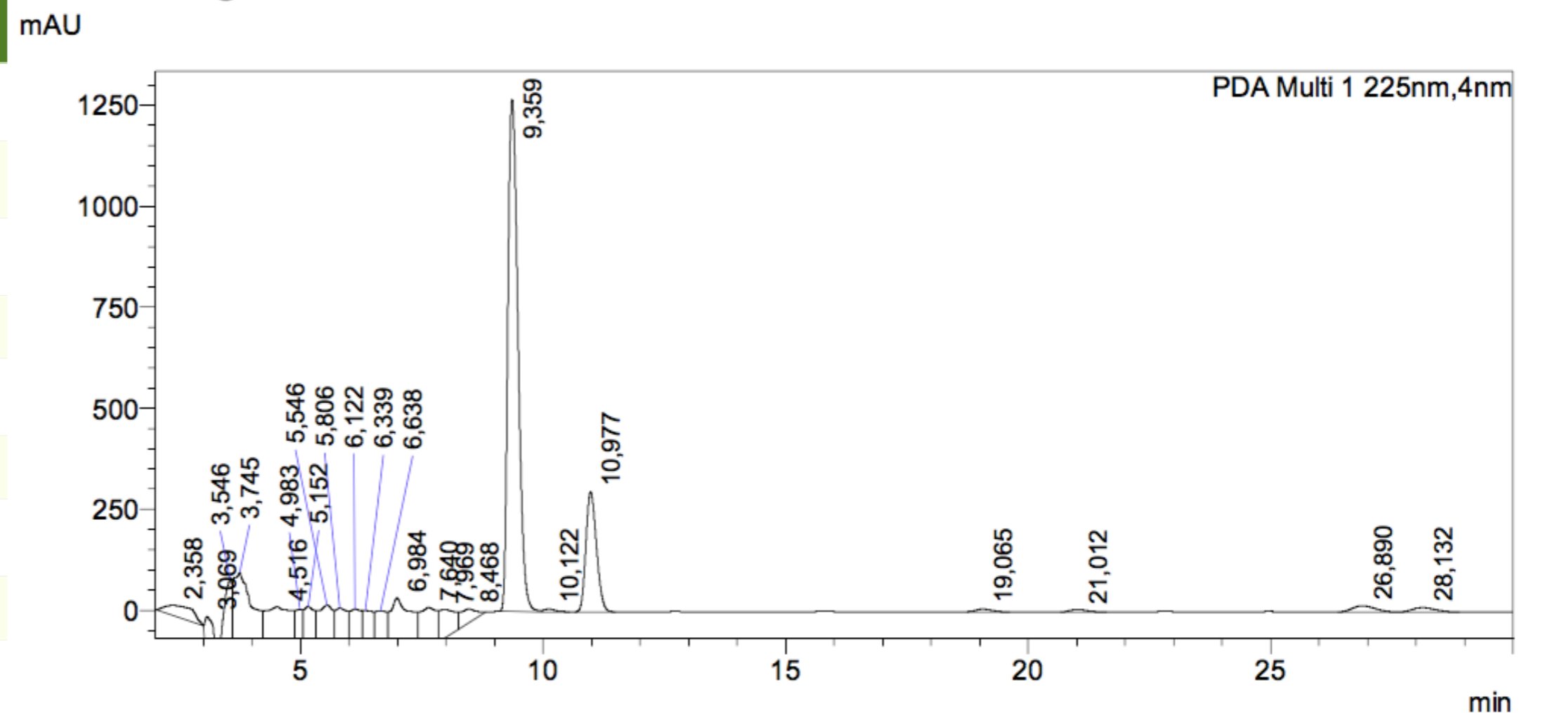
<Chromatogram>
