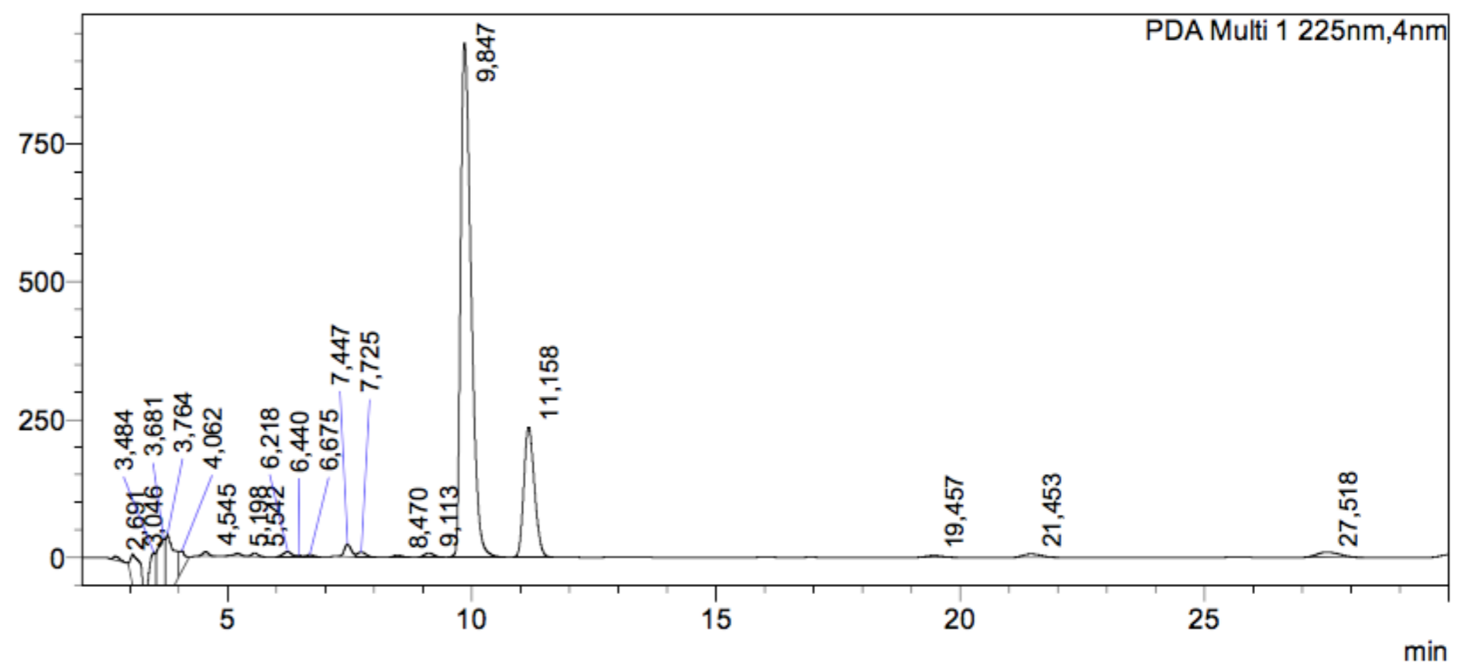
<Chromatogram> mAU
