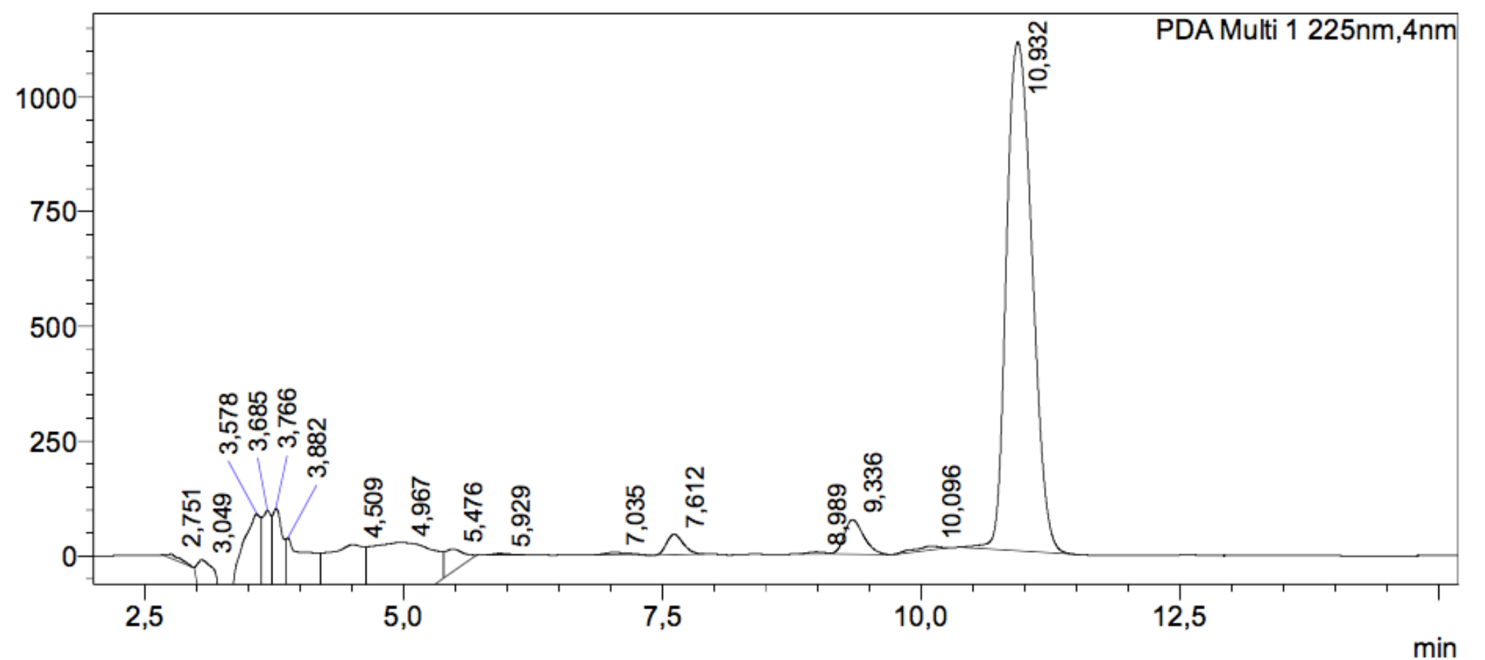
<Chromatogram> mAU
