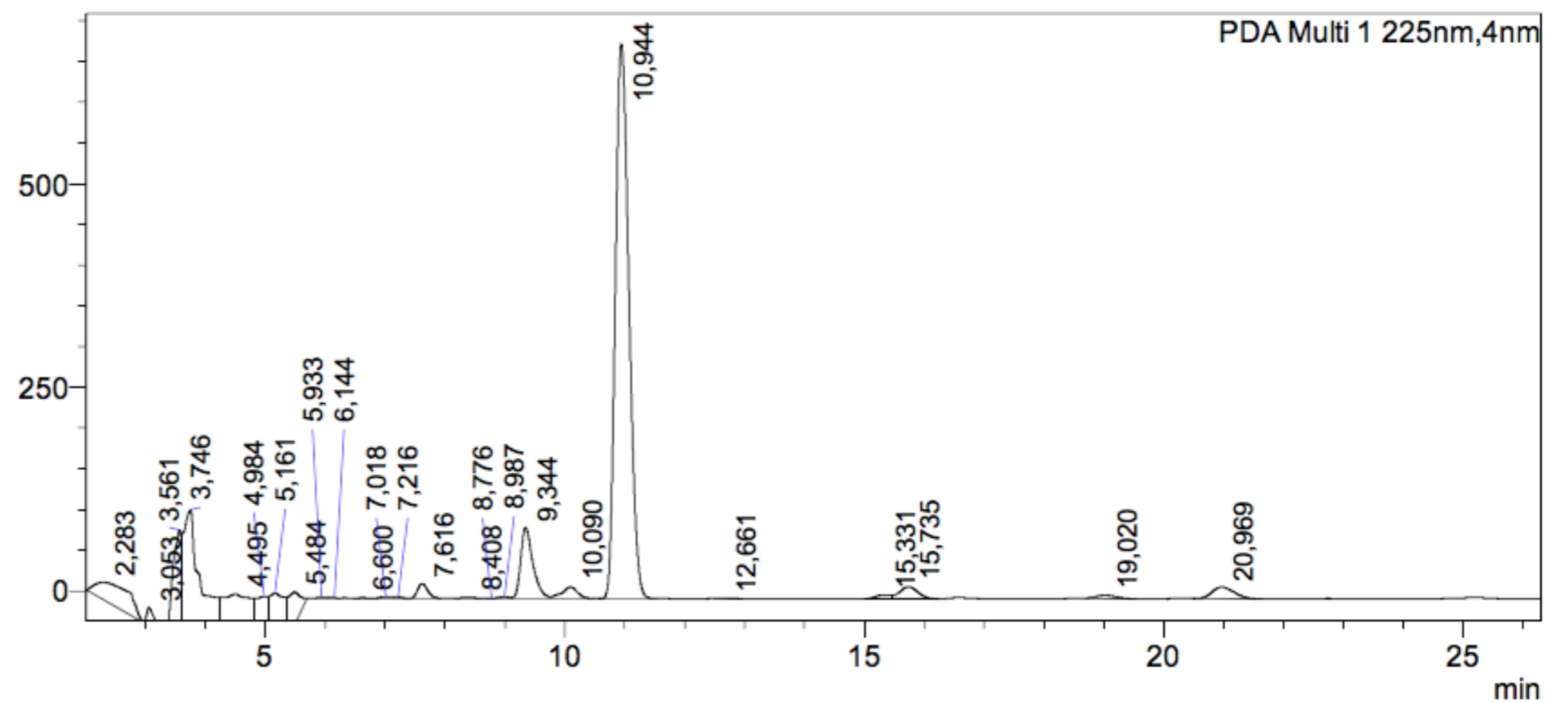
<Chromatogram> mAU
